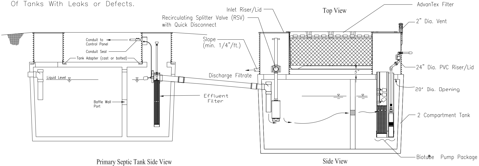
Process Tank
